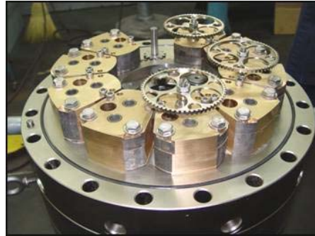
20433 Type 1 CRFD Frame 9FA Flow Divider
